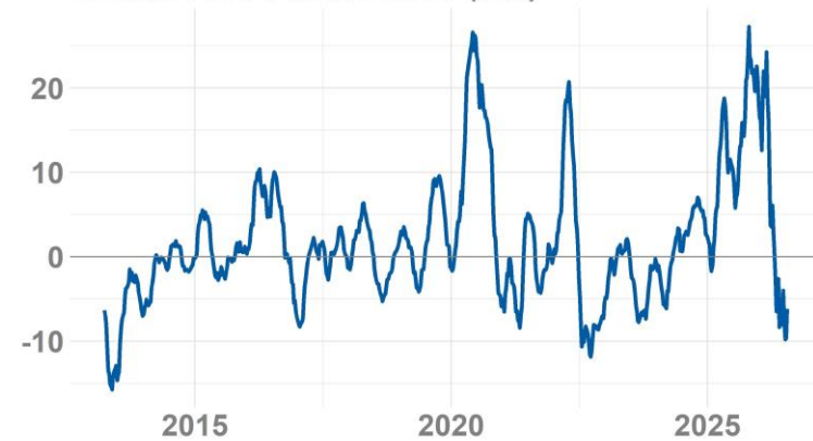
T13wks Flow Commodities ($bn)
